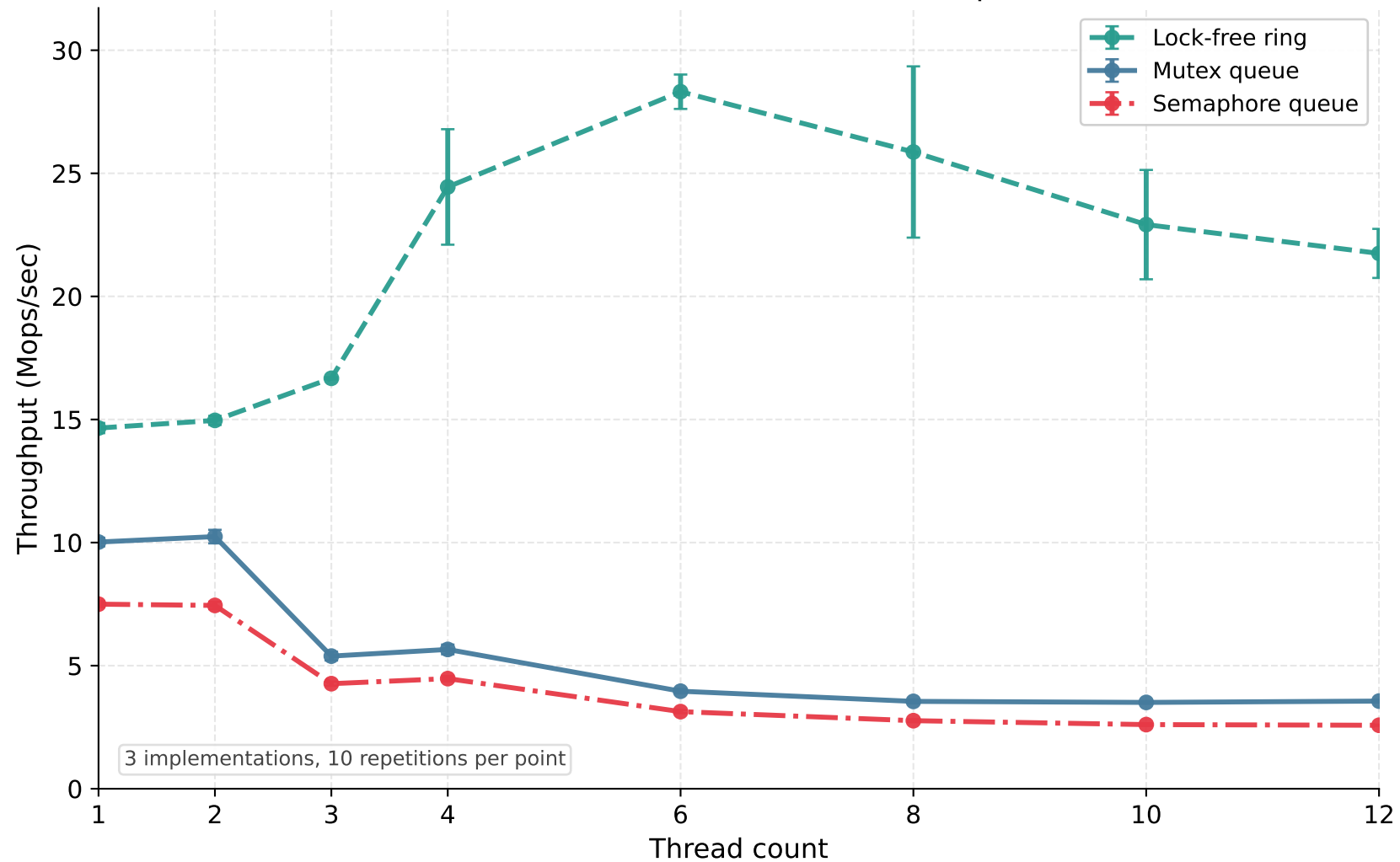
Bounded Producer-Consumer Queue - Balanced producer-consumer
